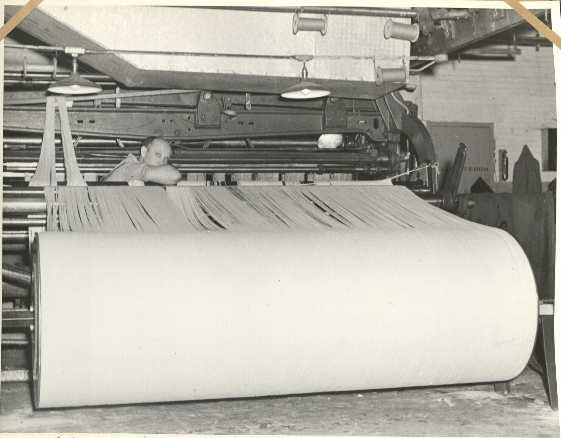
Lacing warps of 8/4 cotton from large 30 inch warp beam at the back of 12/4 converted Axminster loom #33 weaving #4 soft textured Navy duck. Building 11-1 1943 Loom fixer - Harry Freeze
