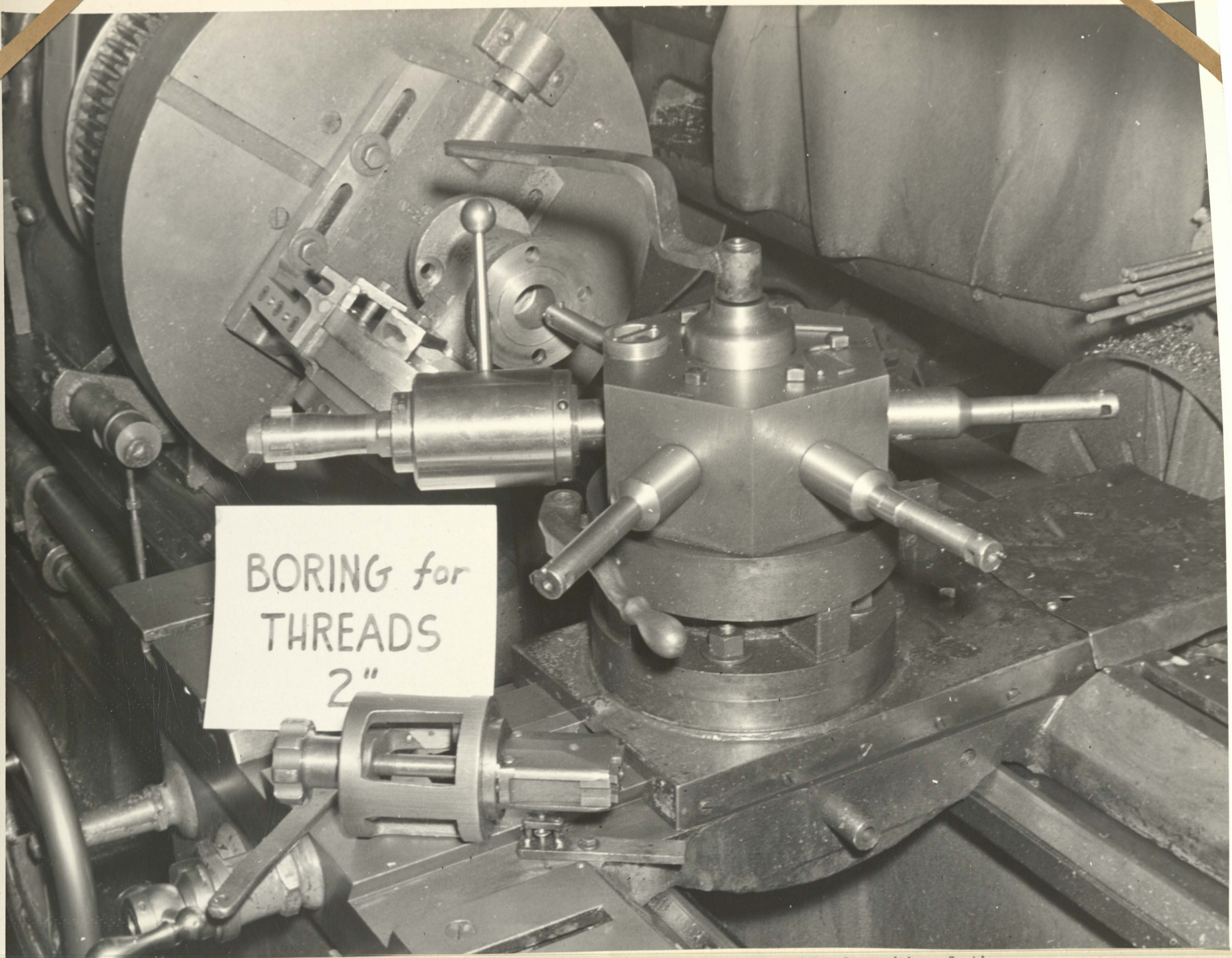
View of turret attachment by The Magee Carpet Company to a Bradford machine lathe. Building 8 - 2 1943
