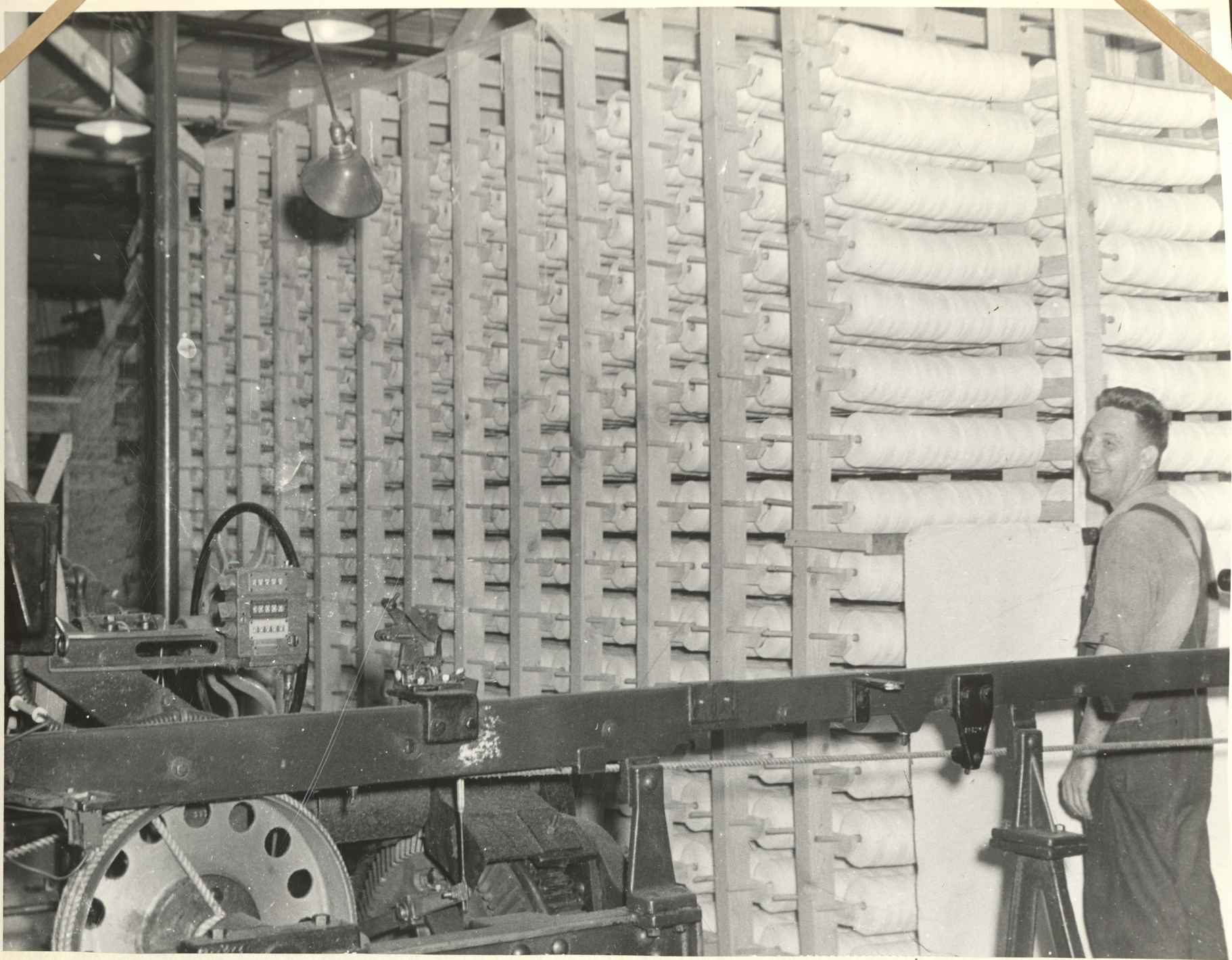
Experimental wooden creel tried to eliminate the beam at the back of a 12/4 Axminster loom weaving 84 inch Navy duck. Creel contains 3150 six by six tubes of cotton yarn. Building 11-1 Loom #9 Fixer - Eugene Derr 1942
