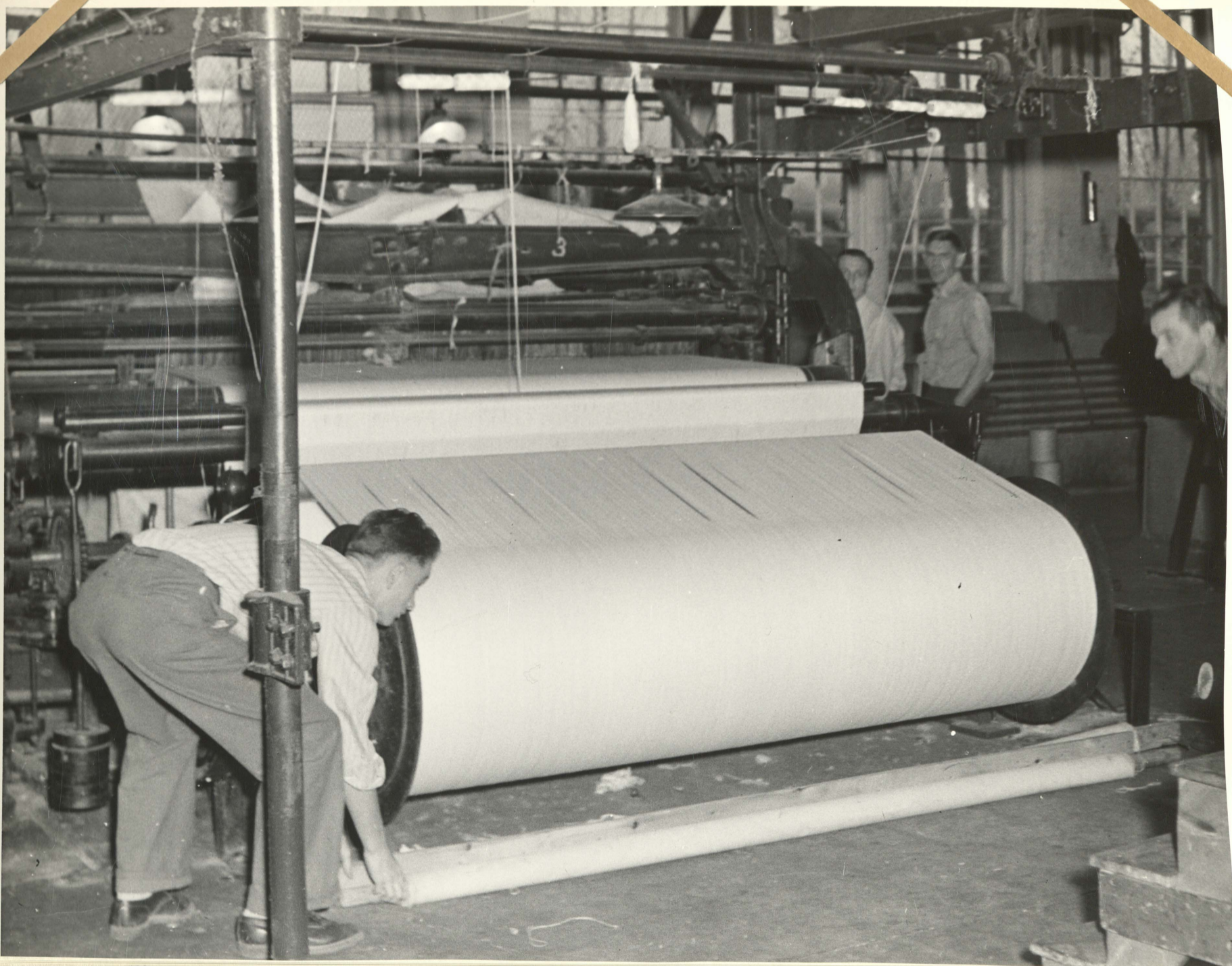
View of large 30 inch diameter 8/4 cotton warp beam for converted 12/4 Axminster loom #6 weaving 84 inch #4 soft medium Navy duck. Building 11-1 1943 Operator - Robert Fought Axminster loom #55 weaving #4 soft textured Navy duck. Building 11-1 1943 Loom fixer - Harry Freeze
