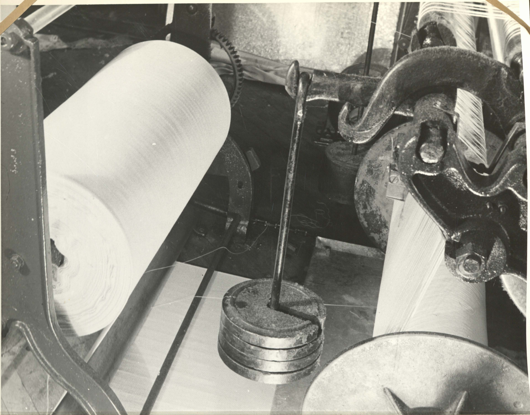
View of sugar bagging cloth on the wind-up roll at the back of a converted 36 inch Axminster loom. Building 12 - 2 1942 36 inch Navy duck. Loom contains 3120 six by six tubes of cotton yarn. Building 11-1 Loom #7 Fixer - Eugene Derr 1942
