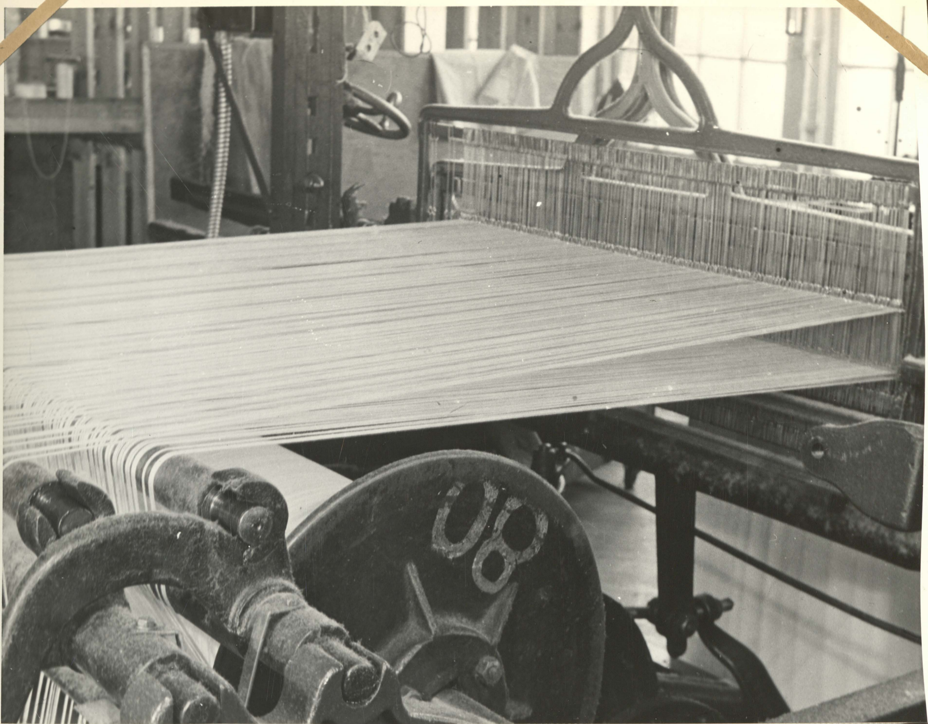
View of back of converted 36 inch Axminster loom weaving sugar bagging cloth. Building 12 - 2 1942
