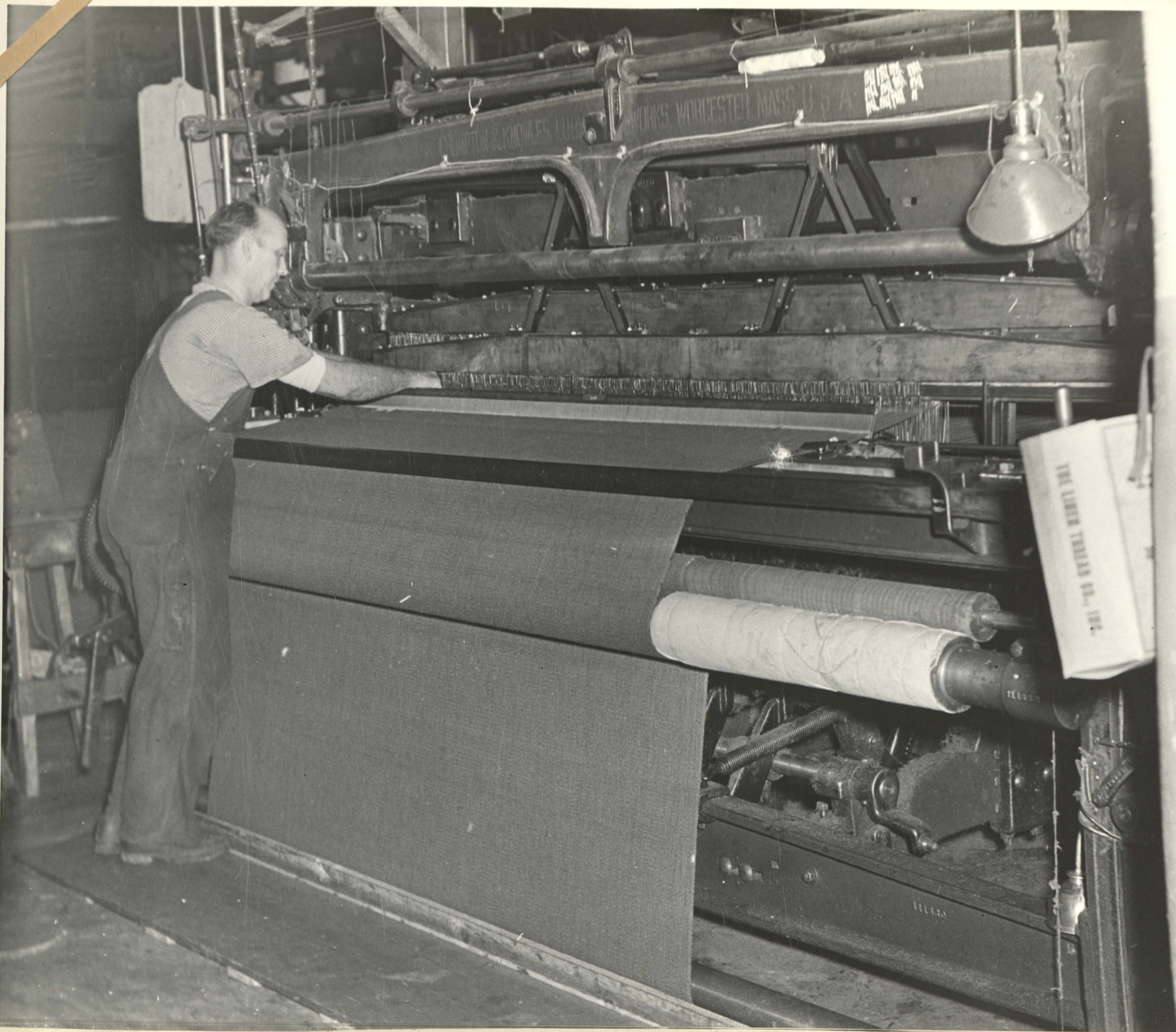
Showing front of converted 12/4 Axminster loom weaving 66 inch all wool Army blanket. Building 11-1 1942 Loom Fixer - Harry Freeze weaving #4 medium soft textured Navy duck. Building 11-1 1942 Operator - Francis Lang Building 11-3 1942
