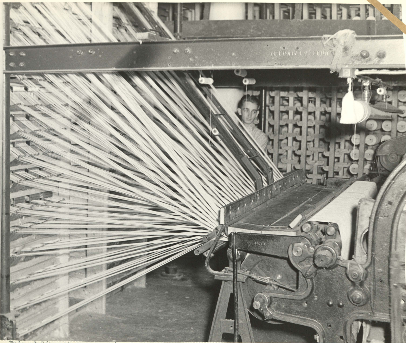
Ends of 8/4 cotton yarn coming from wooden creel and entering let-off roll at the back of a 12/4 Axminster loom weaving 84 inch #4 Medium soft-textured Navy duck. Building 11-1 Loom #8 1942 Operator - Robert Fought, missing in action in Germany December 1944.
