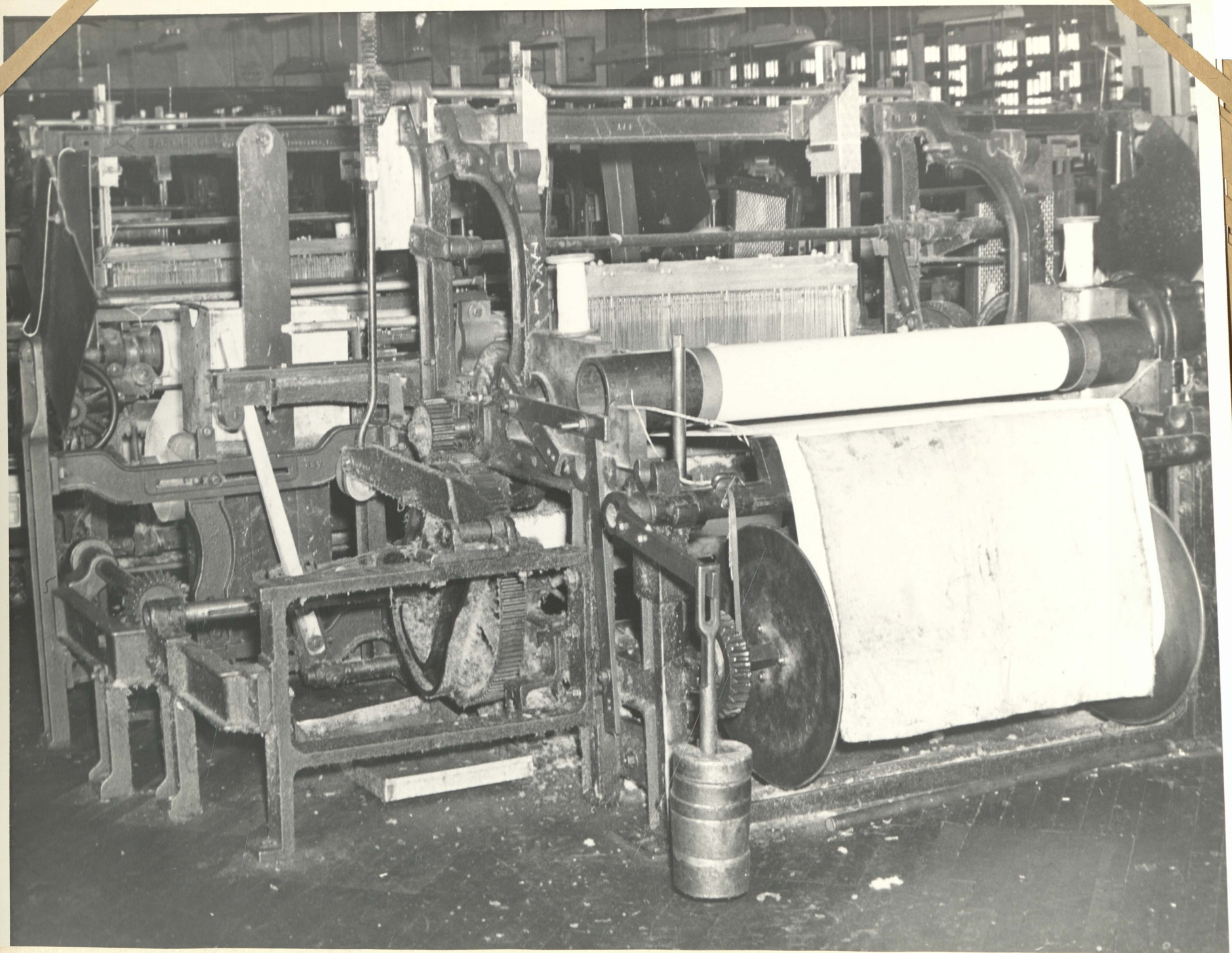
Rear view showing tension rolls and beam of 36 inch Velvet loom converted to the weaving of #6 - 37 inch Army duck. Building 11-3 1942
