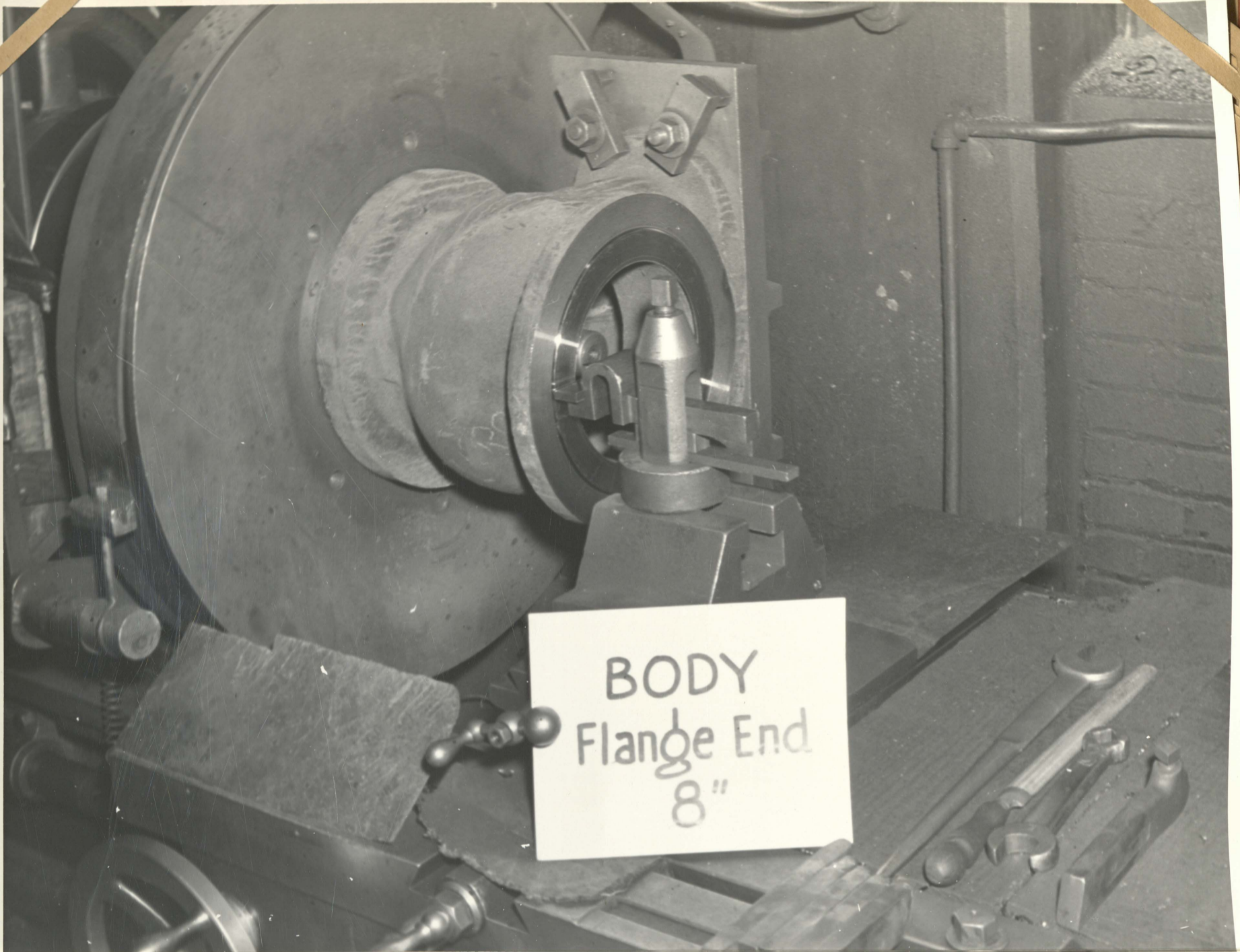
Fay and Scott machine lathe Building 8 - 2
