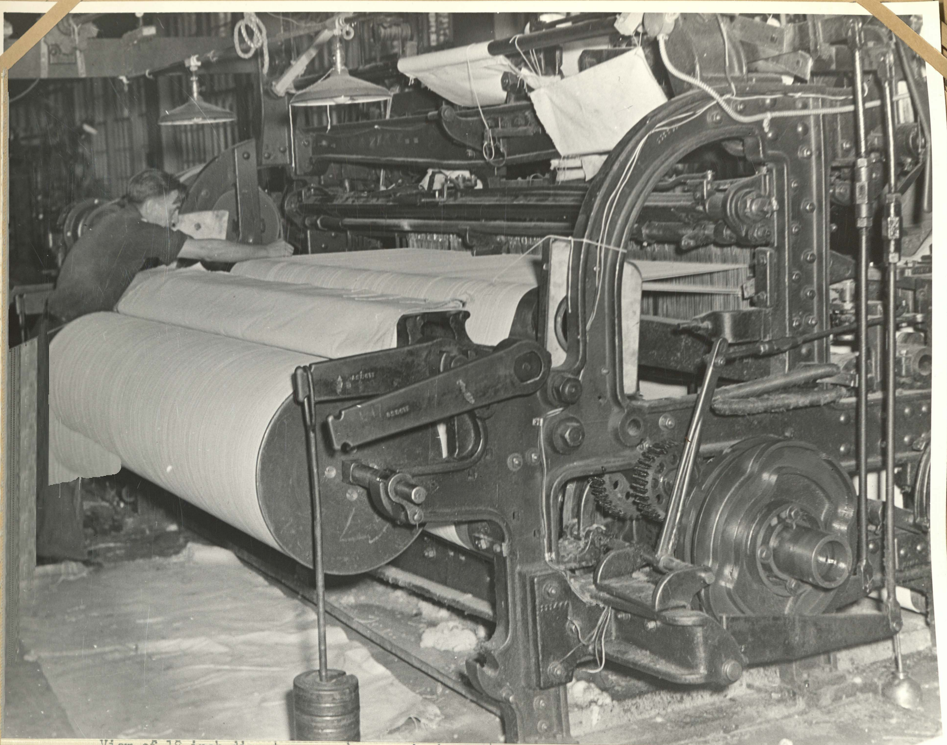
View of 18 inch diameter warp beam on back of first converted 12/4 Axminster loom for weaving #4 medium soft textured Navy duck. Building 11-1 1942 Operator - Francis Lang
