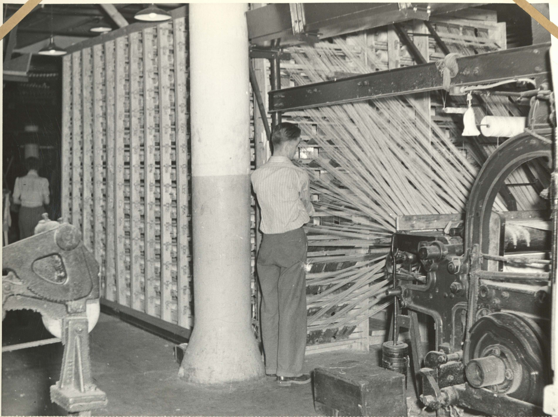
View of wooden creel at the back of converted 12/4 Axminster loom weaving 84 inch Navy duck. Creel contains 3150 six by six tubes of 8/4 cotton yarn. Duck was #4. Medium soft texture with 7/4 filling. Building 11-1 Loom #8 1942 Operator - Robert Fought, missing in action in Germany December 1944.
