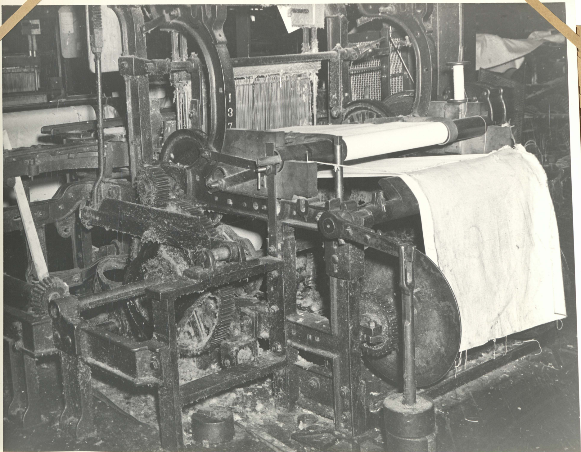
Side view of 3/4 Velvet loom converted to the weaving of #6 - 29 inch Army duck. Building 11-3 1942
