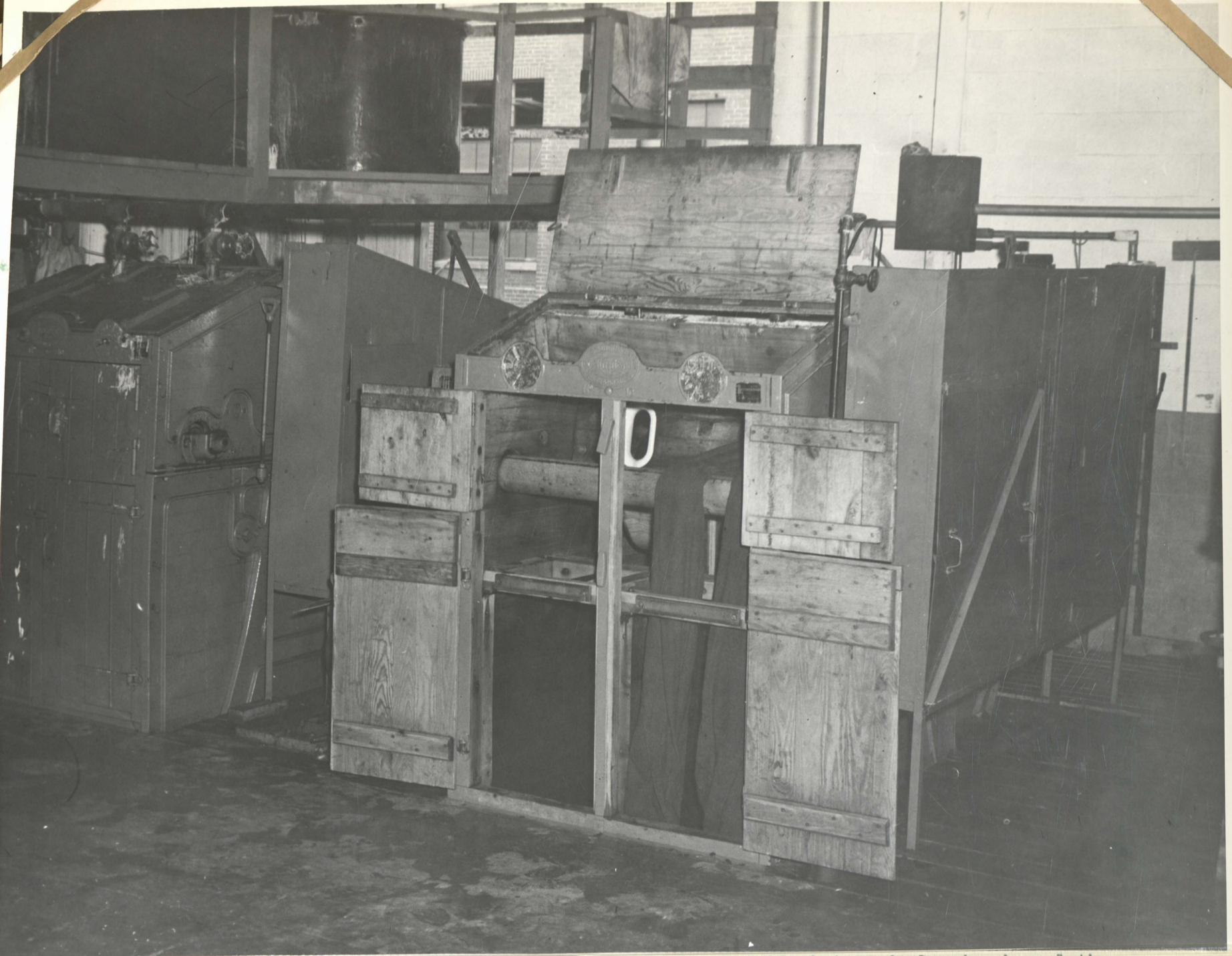
View of James Hunter fulling machine used for fulling Army blankets and sleeping-bag cloth. Building H 1943
