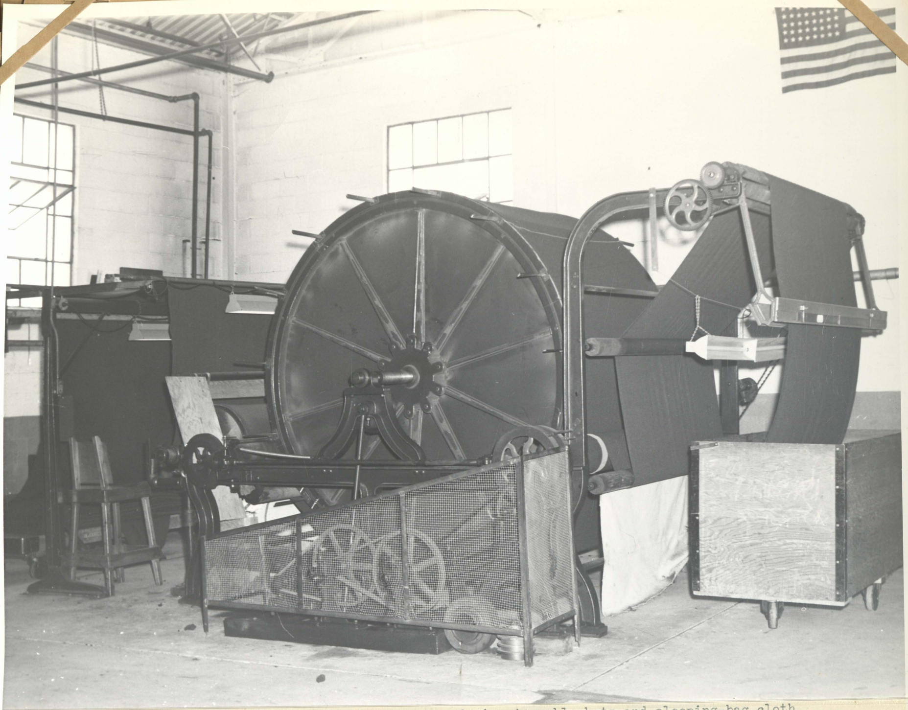
Side view of Curtis and Marble dryer used for drying Army blankets and sleeping-bag cloth. Building H 1943 Building H 1943
