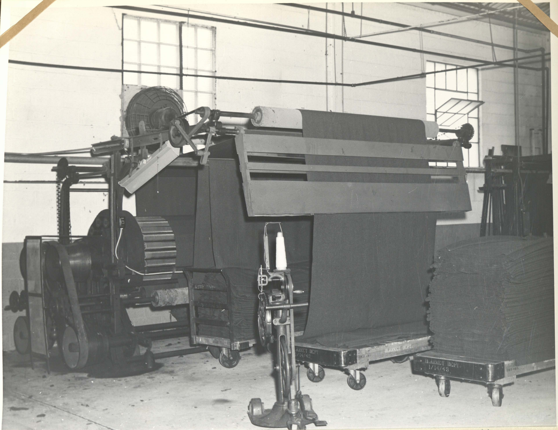
Picture of Davis and Furber break napping machine. This is a 24 roll double action machine. Building H 1943
