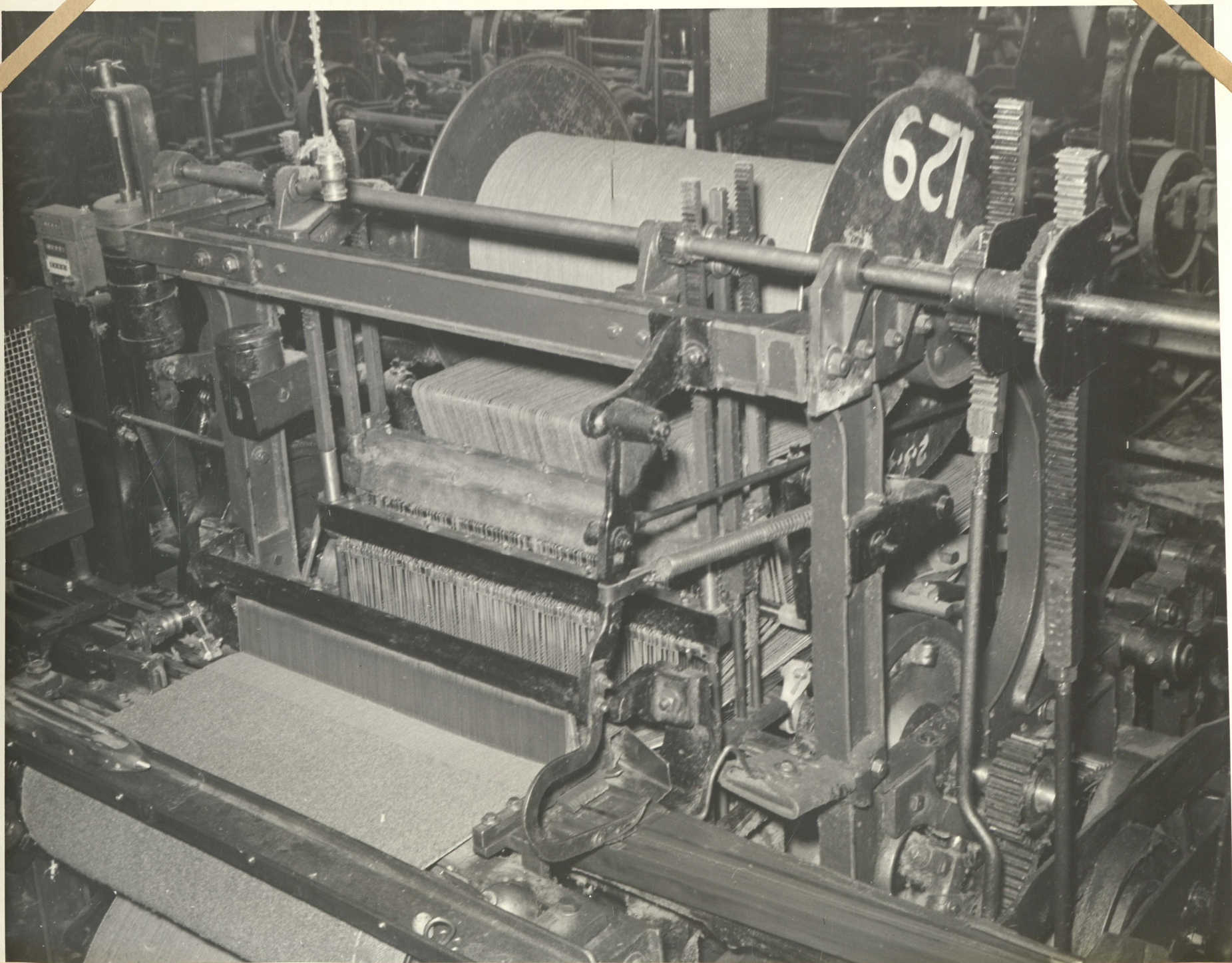
Front view of 3/4 Velvet loom new type or rack motion for heddle frames. Note elimination of old style jack arms. Building 11-3 1944
