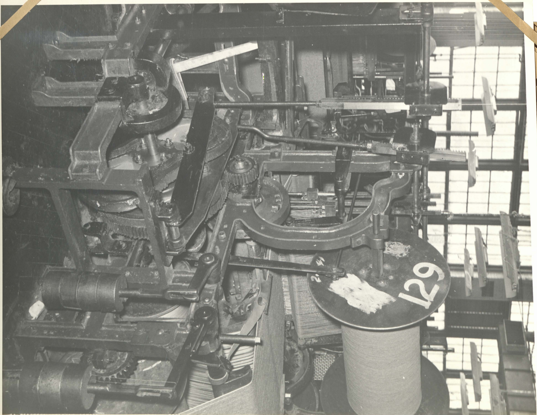
Side view of 3/4 Velvet loom showing new type or rack heddle motions replacing inefficient jack arms. Building 11-3 1944 of old style jack arms. Building 11-3 1944
